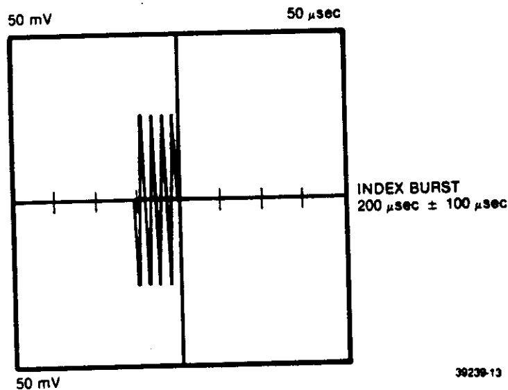
FIGURE 5-10. INDEX BURST
