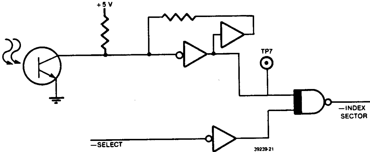
FIGURE 4-9. INDEX DETECTOR
