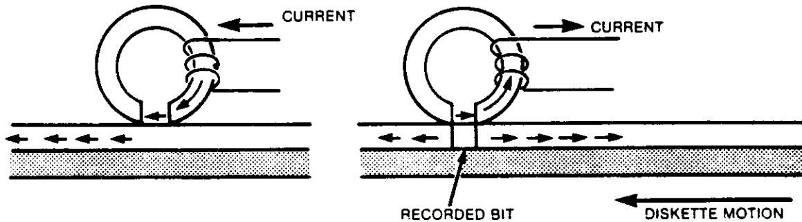
FIGURE 4-3. RECORDED BIT
