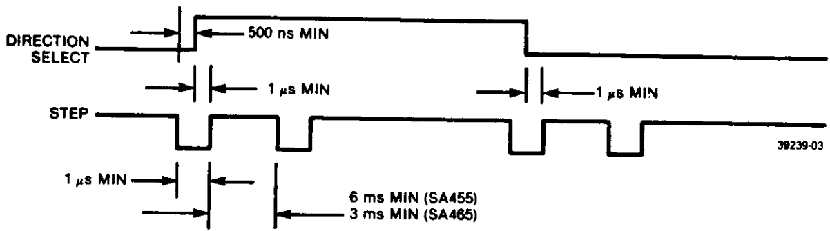
FIGURE 4-10. STEPPER TIMING
