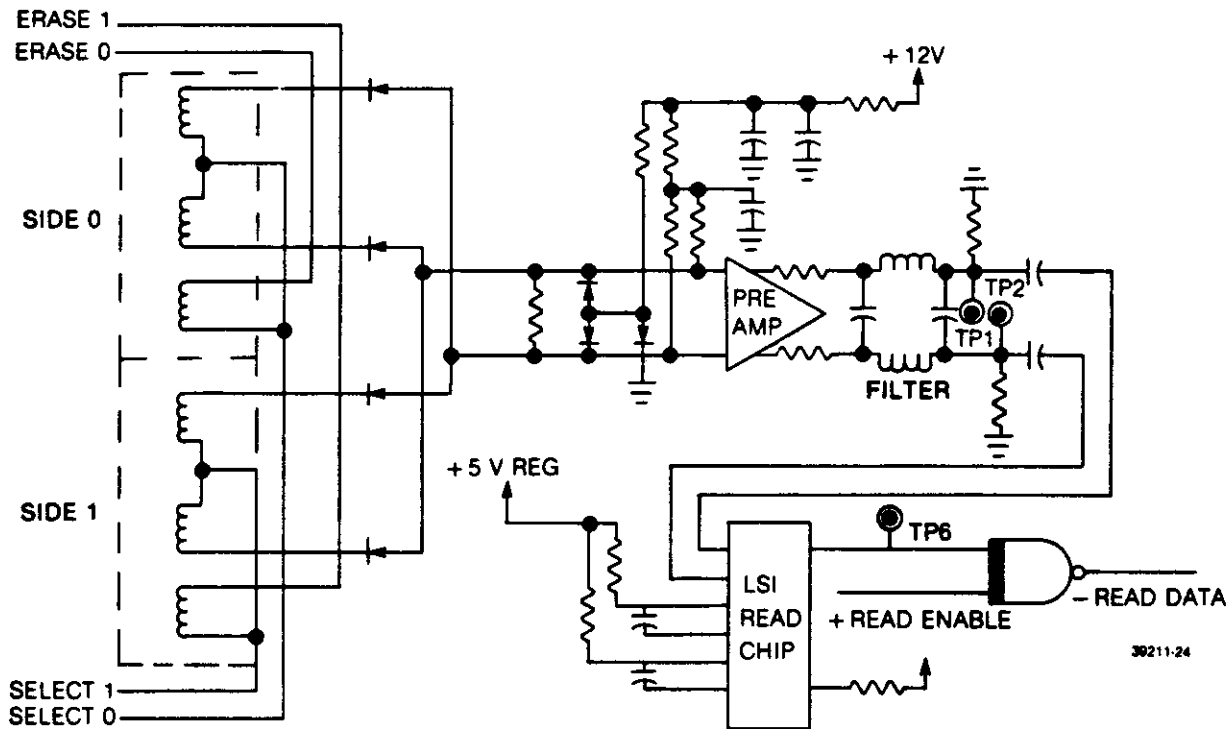
FIGURE 4-8. READ CIRCUIT
