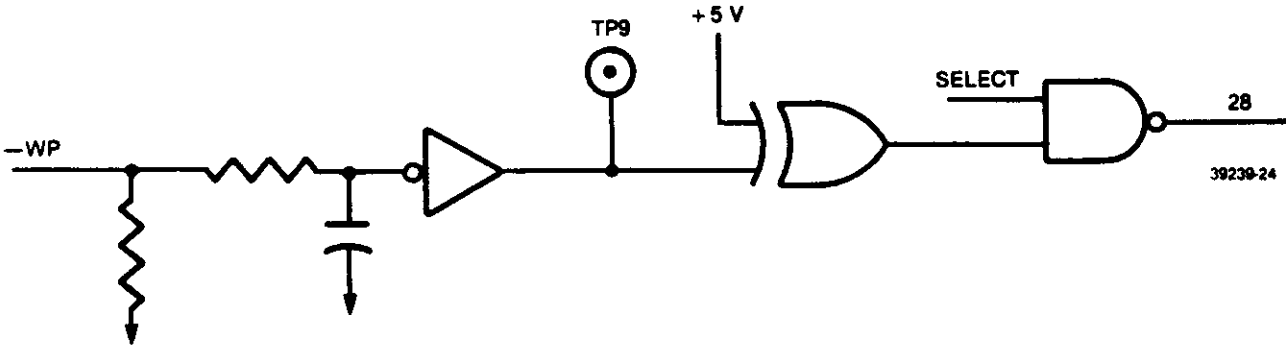
FIGURE 4-13. WRITE PROTECT
