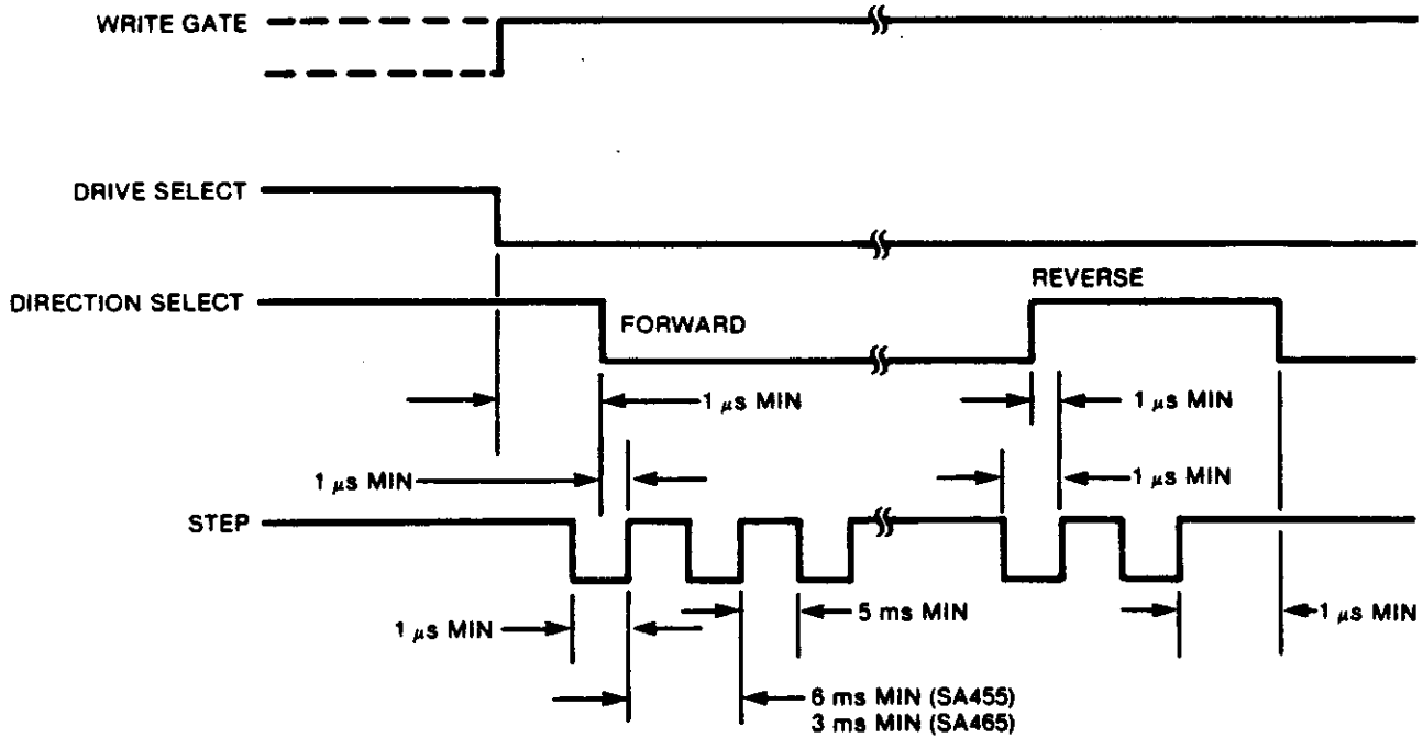
FIGURE 2-3. STEP TIMING
