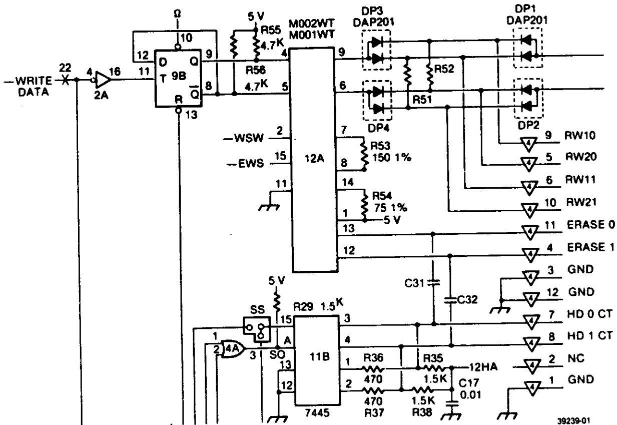
FIGURE 4-7. WRITE CIRCUIT
