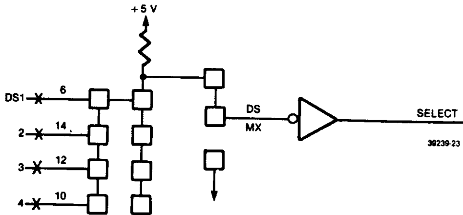
FIGURE 4-12. DRIVE SELECT
