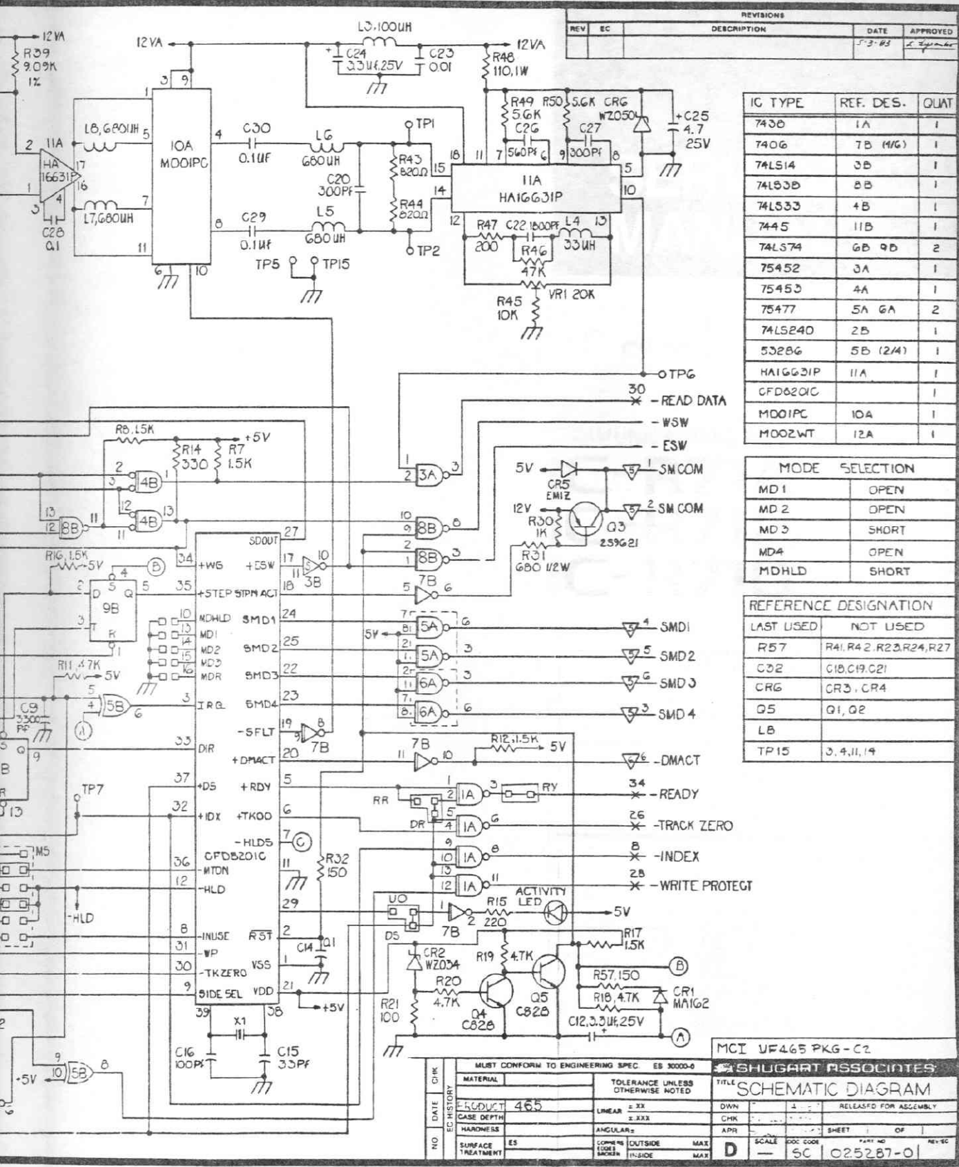
FIGURE 6-2. SCHEMATIC DIAGRAM, P/N 25286
