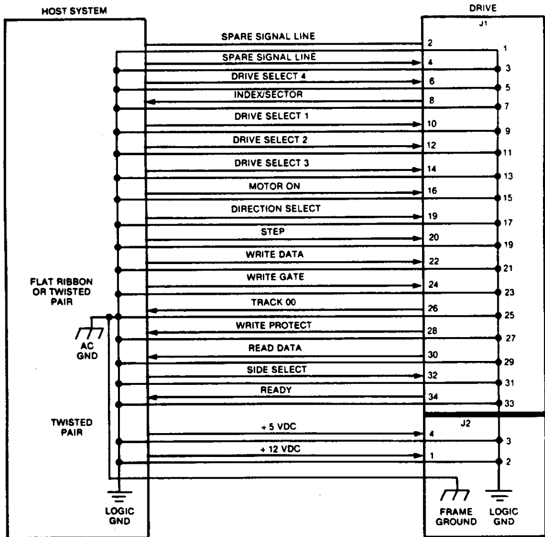
FIGURE 2-1. INTERFACE CONNECTIONS
