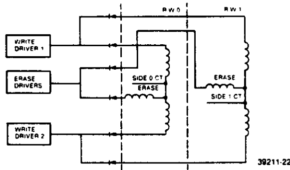
FIGURE 4-6. READ/WRITE HEADS
